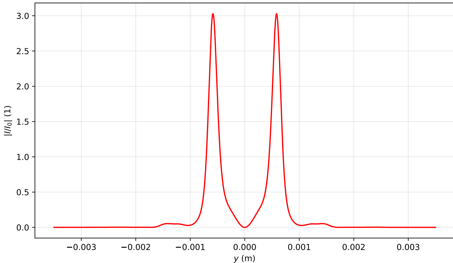
Intensity profile I(x=0, y, z=1.194)/I_0 , P_{in}=9.0P_{cr} , artificial time
